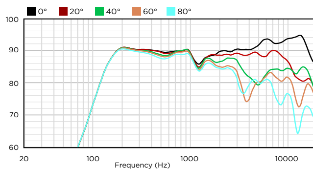
OFF-AXIS RESPONSE (dB SPL) 9
