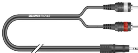
Cablu adaptor RCA la Jack Stereo Sommer BV-CIJ3-0075, 0.75m, 2xRCA, 1xJack Stereo (3.5mm)
