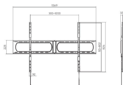
Dimensions (mm)
