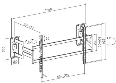
Dimensions (mm)
