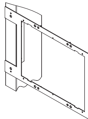
Pre-Construction Mount Kit (PMK)
