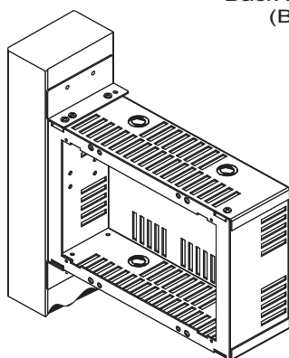
Side mount Installations
