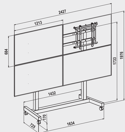
MOVYALL-H 2X2 cod. 07095 Single Side cod. 08008 BackToBack
