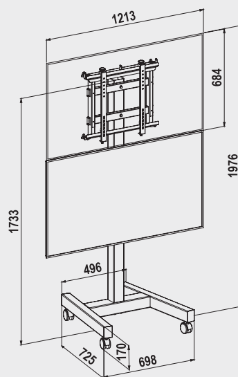
MOVYALL-H 2X1 cod. 08004 Single Side cod. 08009 Back to Back
