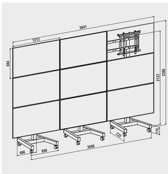
MOVYALL-H 3X3 cod. 08001 Single Side cod. 08006 Back to Back
