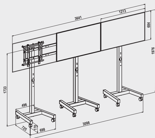
MOVYALL-H 1X3 cod. 08003 Single Side cod. 08010 Back to Back
