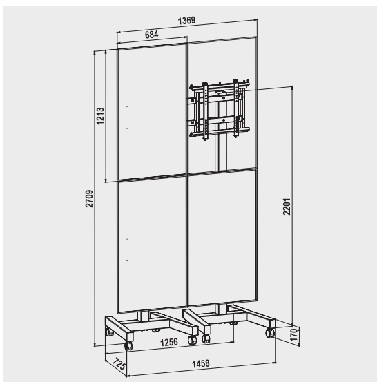
MOVYALL-V 2X2 cod. 08030 Single Side
