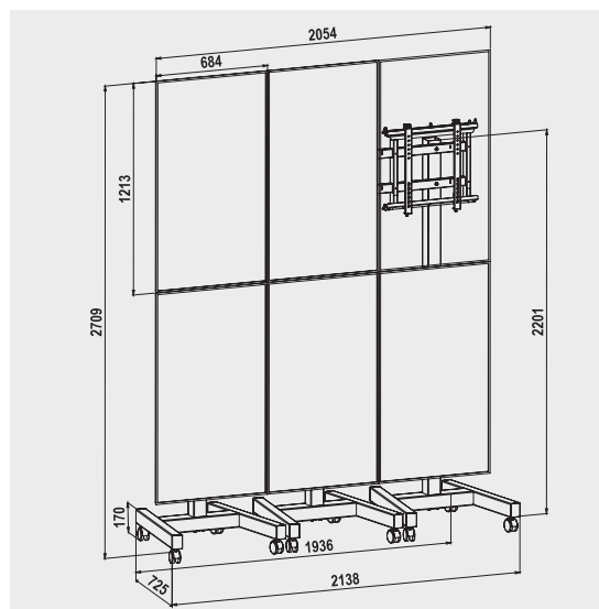
MOVYALL-V 2X3 cod. 08031 Single Side
