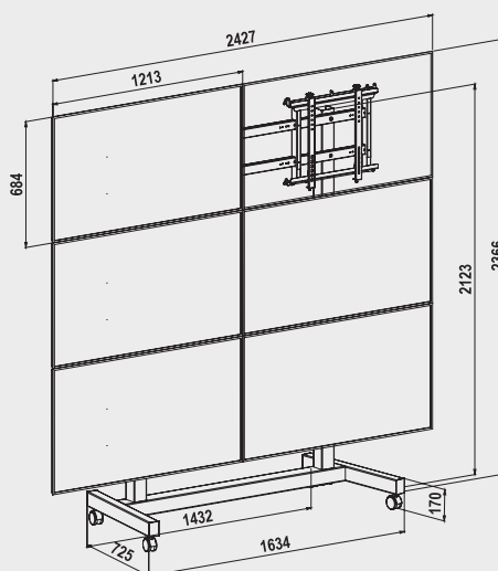
MOVYALL-H 3X2 cod. 08005 Single Side cod. 08007 BackToBack
