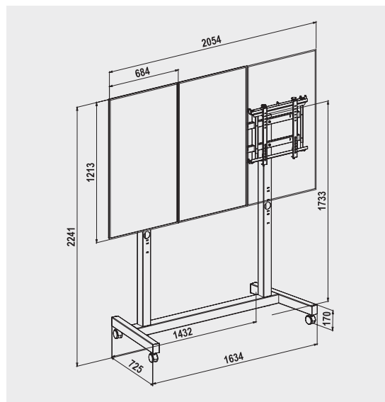
MOVYALL-V 1X3 cod. 08029 Single Side
