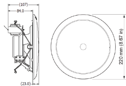
LC1-UM24E8 Dimensions in mm
