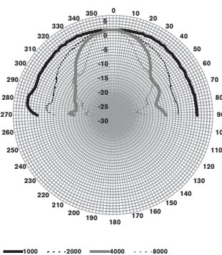
LC1-UM06E8 Polar diagrams
