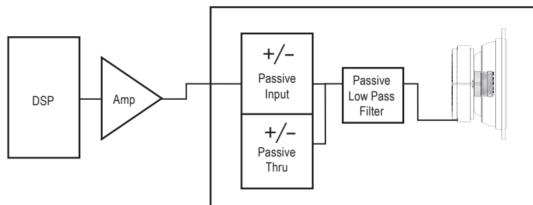
Single amp
