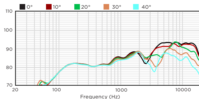
VERTICAL OFF-AXIS DOWN RESPONSE (dB)
