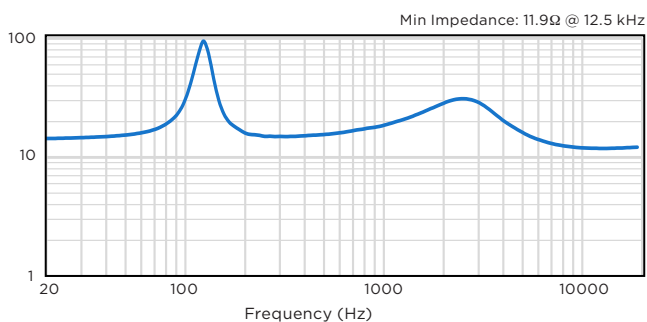
IMPEDANCE (Ohms)
