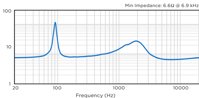
IMPEDANCE (Ohms)
