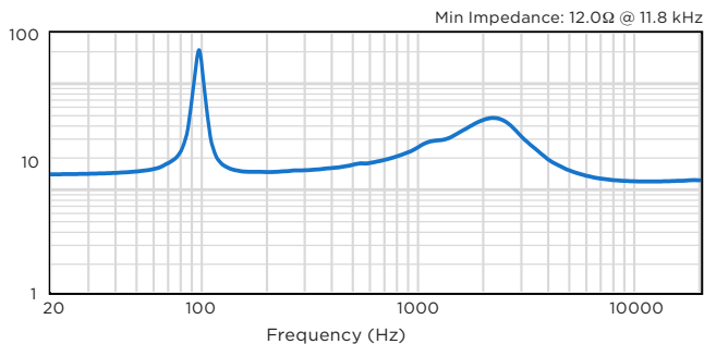
IMPEDANCE (Ohms)
