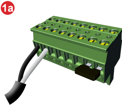
1a Low Impedance operation (move preinstalled jumper to unused terminals)
