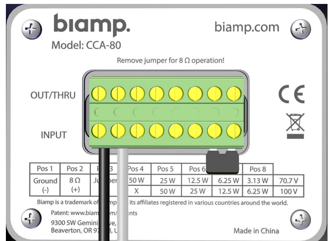
Cabinet - independently wired (or last cabinet in series)
