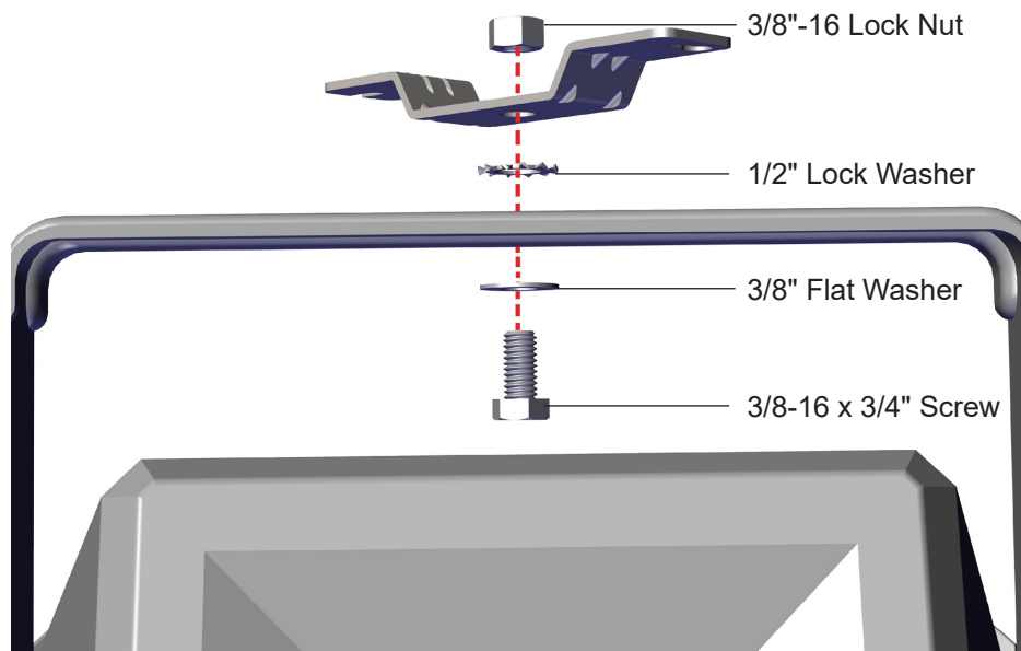
Figure 10. Bracket install
