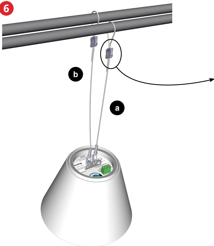
Allow slack in secondary cable (b) so pendant hangs straight
