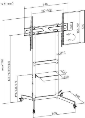
Dimensions (mm)
