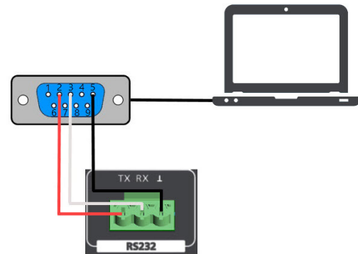
Figure 18. RS232 Wiring
