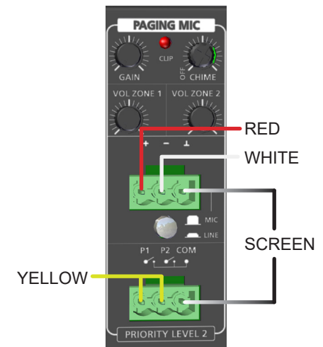
Figure 4b. MICPAT-D Wiring
