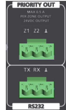
Figure 9. Priority Out & RS232
